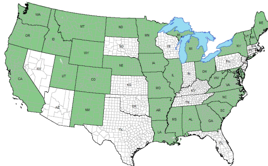
2009 NAIP COVERAGE
