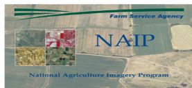
2005 NAIP COVERAGE
