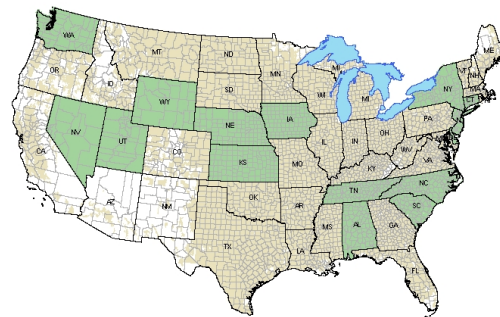
2006 NAIP COVERAGE
