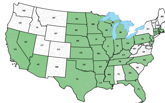
2010 NAIP COVERAGE
