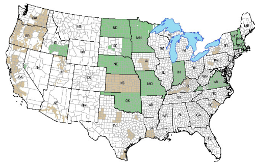
2003 NAIP COVERAGE
