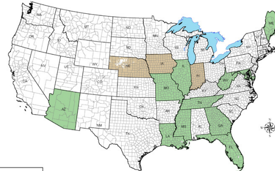
2007 NAIP COVERAGE
