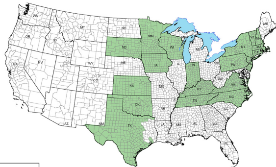
2008 NAIP COVERAGE
