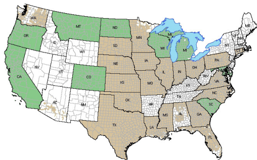
2005 NAIP COVERAGE
