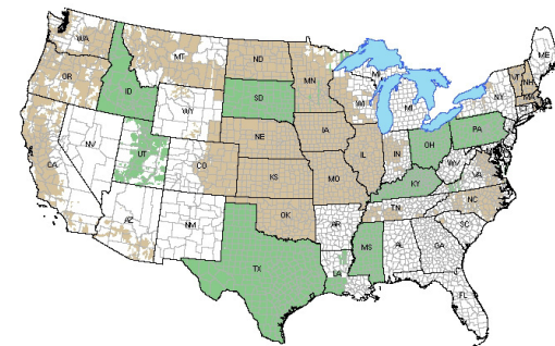
2004 NAIP COVERAGE
