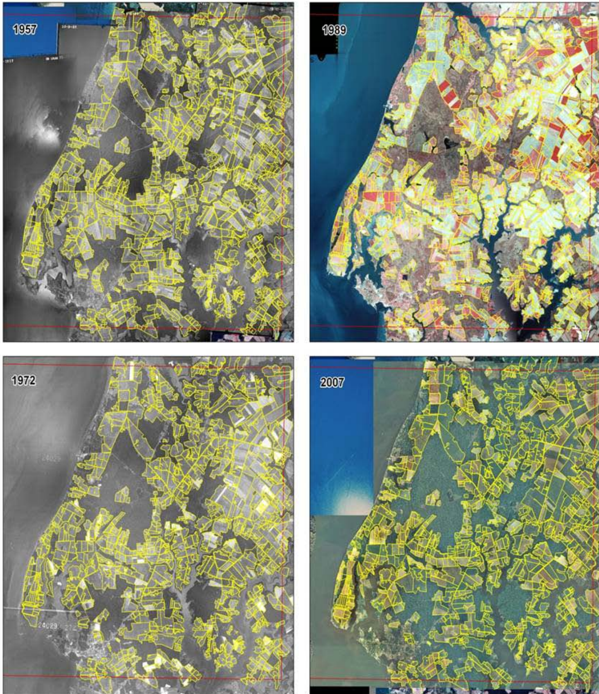
Figure 5: A time series study showing the loss of agricultural land. Agricultural polygons were hand digitized
