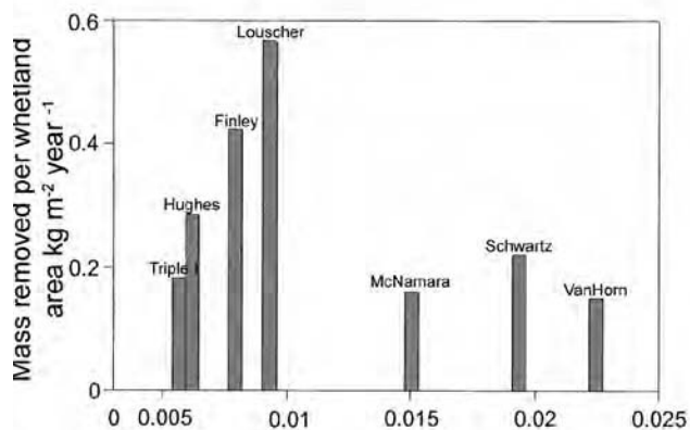
Figure 15. Predicted mass nitrate removed per area of wetland as a function of wetland/watershed area ratio.
