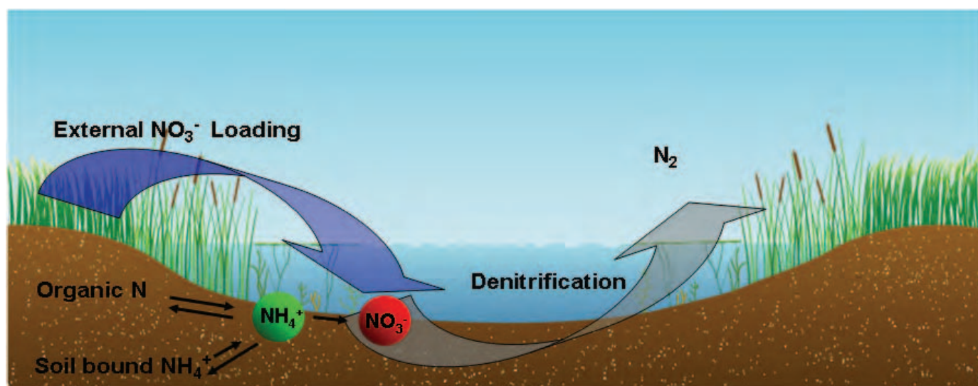
Figure 6. Simplified representation of nitrogen transformations in wetlands illustrating the increased importance of denitrification in wetlands receiving significant external nitrate loads (not all transformations are shown).
