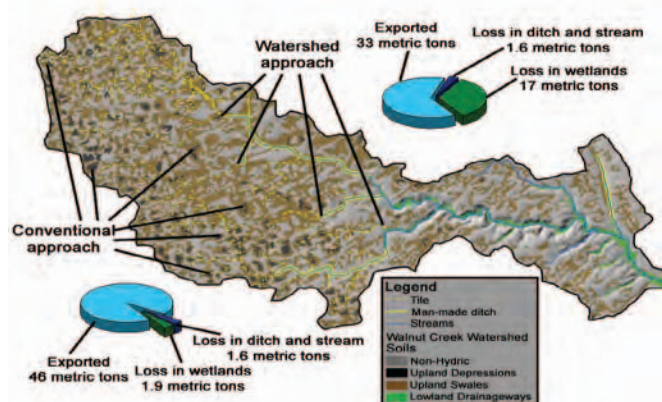
Figure 9. Annual nitrate mass balance for Walnut Creek watershed under alternative wetland restoration scenarios (conventional approach versus watershed approach).
