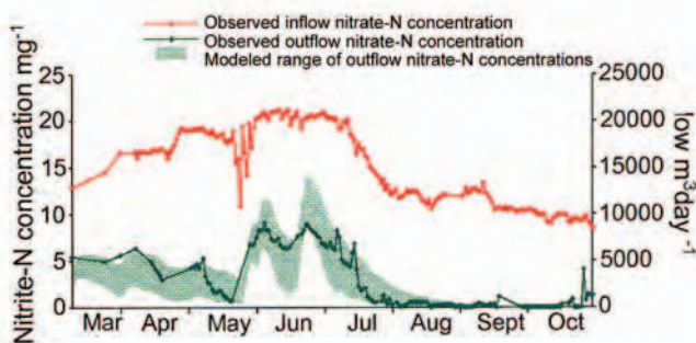
Figure 12. Modeled and observed nitrate concentrations for Van Horn Wetland in 2004.
