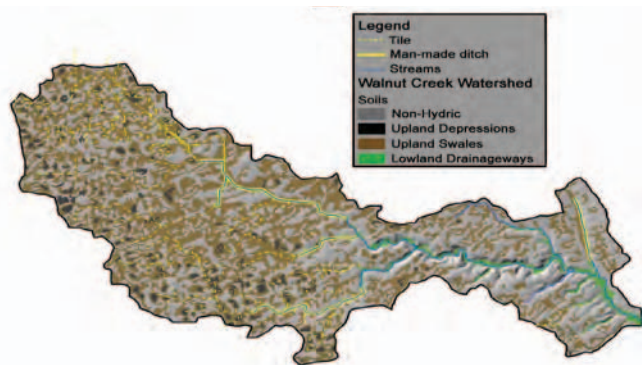
Figure 8. Current surface and subsurface drainage systems in Walnut Creek watershed and presettlement distribution of wetlands estimated from hydric soils (upland depressions, upland swales, and lowland drainageways). Soil distribution derived from the Iowa Cooperative Soil Survey.
