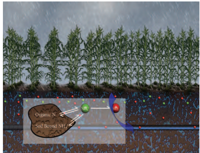
Figure 3. Simplified representation of nitrogen transport in tile drained cropland illustrating nitrate leaching and transport with infiltrating water during a rain event.
