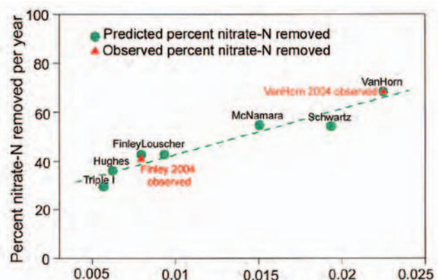
Figure 14. Predicted and observed percent nitrate removed as a function of wetland/watershed area ratio.
