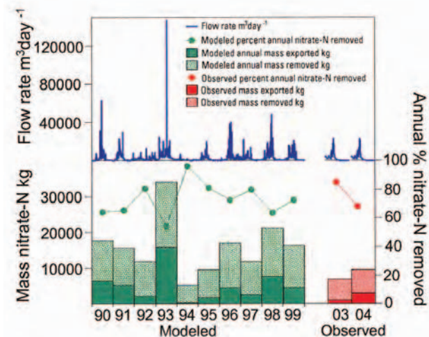
Figure 13. Percent nitrate removal and nitrate mass balance for Van Horn Wetland modeled for 1990–1999 (annual) and observed for 2003 and 2004 (field season).
